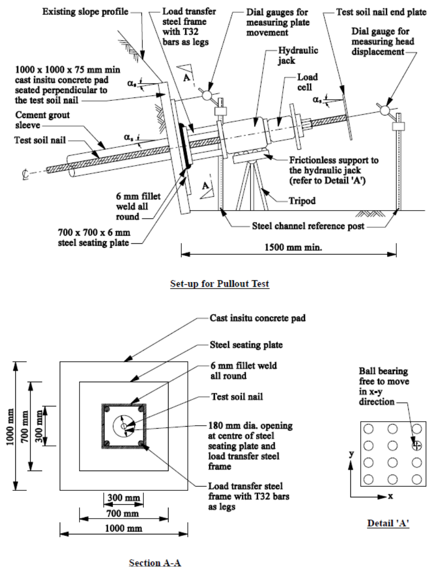
Figure 701-1: Pull-out test arrangement
