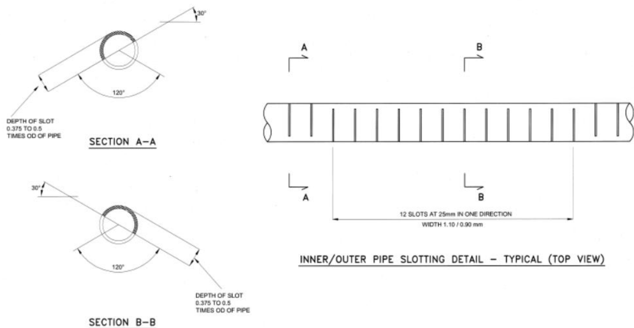
Figure 702-2: Horizontal Drain Perforation/slotting Detail
