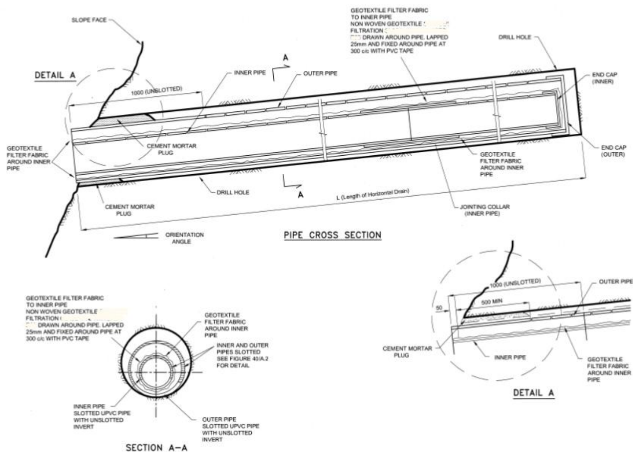
Figure 702-1: Type 3 – Horizontal Drain Detail
