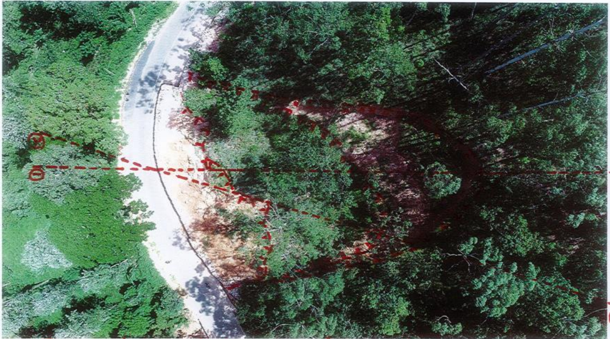
Figure 3: Drone image of the proposed landslide mitigation site, the surrounding environmental features and service infrastructure
