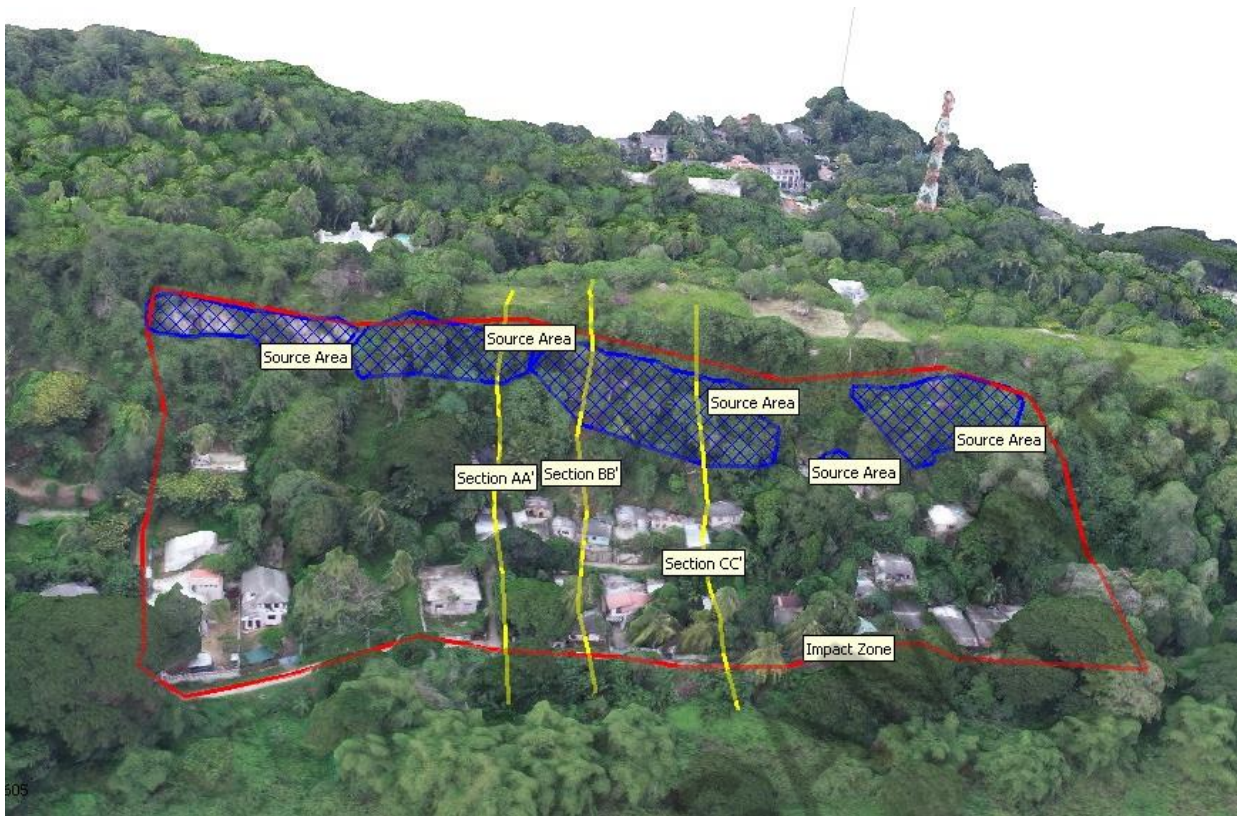
Fig. 3.2: Sectional view of the Drone image of the area
